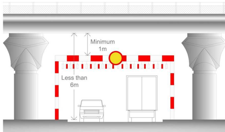
Figure 7.1: Site Preparation – Temporary Traffic Access
