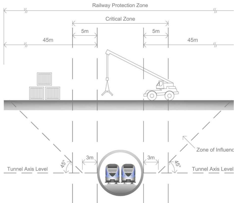
Figure 4.1: RA1.1 - Loads imposed by placing or using heavy machinery or goods above Railway structures should be checked against the allowable limits
