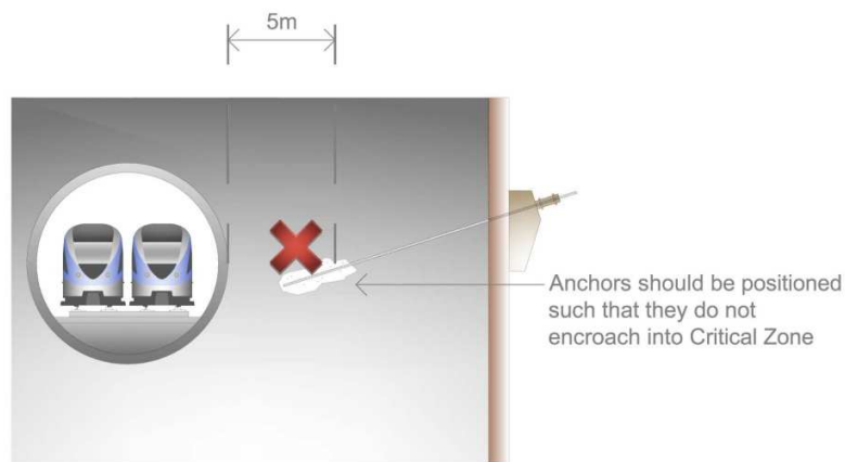
Figure 7.5: Ground Anchor Restrictions
