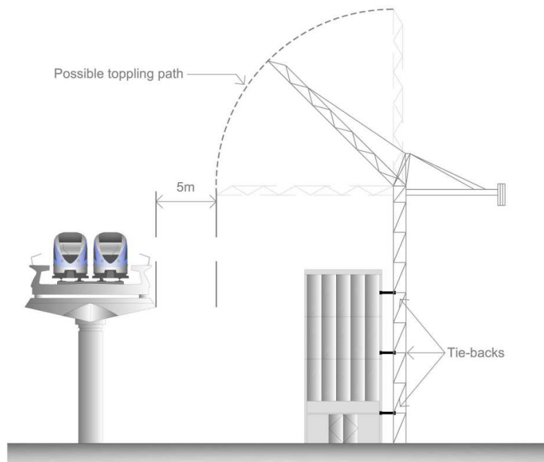
Figure 4.5: RA2.3 - Tower crane and its parts erected behind building and tied back, should topple outside the Critical Zone
