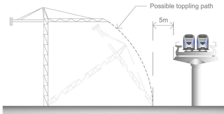
Figure 4.6: RA2.4 - Free standing tower crane or its parts should not topple inside the Critical Zone
