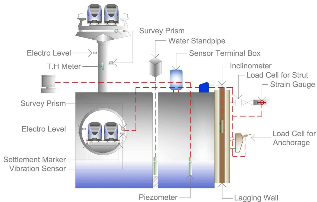
Figure 8.1: Typical Monitoring Scheme
