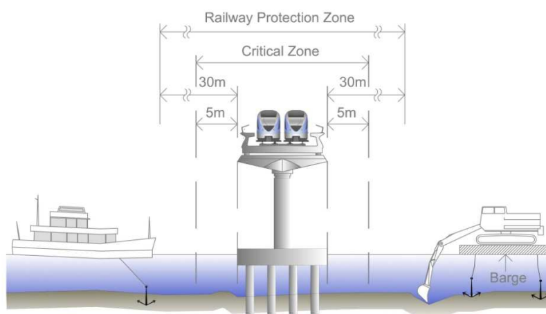
Figure 4.9: RA4.2 - Anchoring of vessels and dredging should be outside the Railway Protection Zone for bridges
