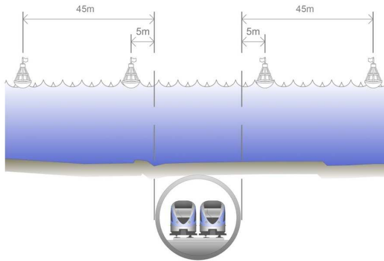
Figure 7.3: Site Preparation – Marine Works Site above Railway Tunnels
