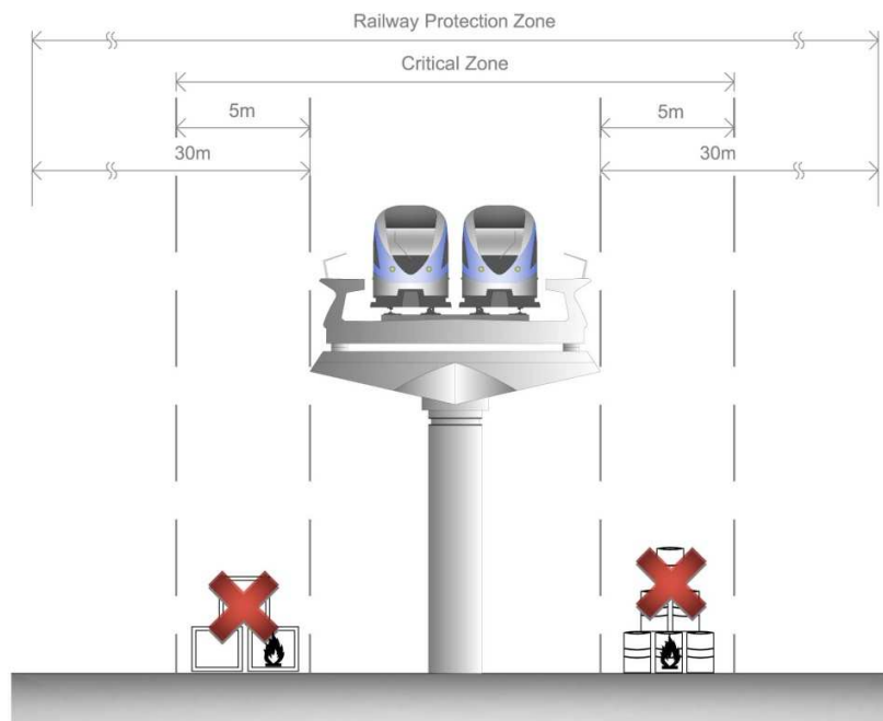
Figure 4.2: RA1.2 - All flammable, combustible or explosive goods such as tankers, fuel containers, and gas cylinders should be kept outside the Critical Zone
