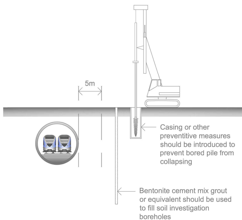
Figure 4.7: RA3 - Boreholes and piles should be outside the Critical Zone and should be checked for potential impacts on Railway structures
