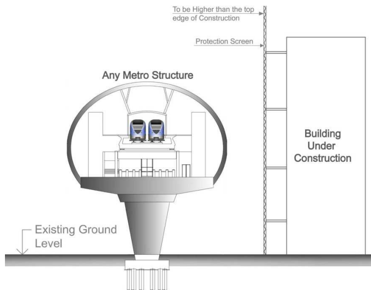
Figure 4.14: RA9.2 - Installation of Protection Screen for Building Under Construction
