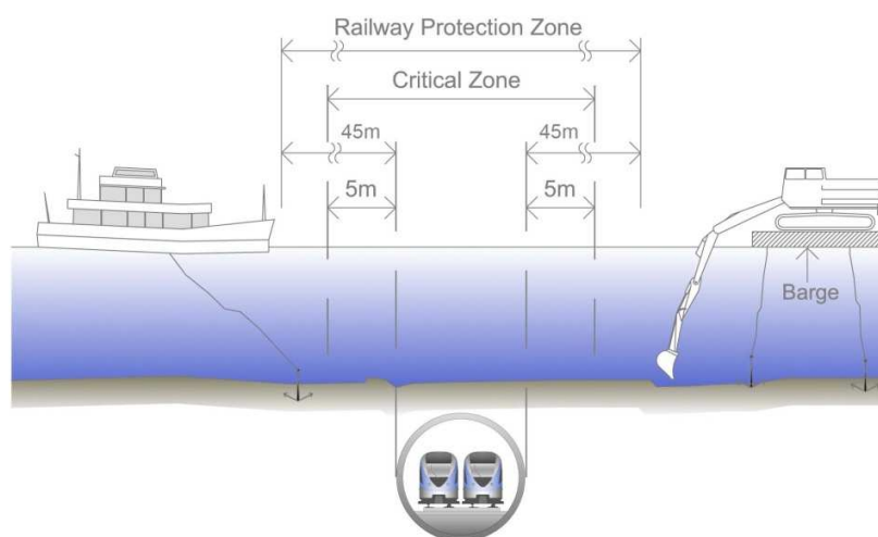
Figure 4.8: RA4.1 - Anchoring of vessels should be outside the Critical Zone and dredging should be outside the Railway Protection Zone for tunnels
