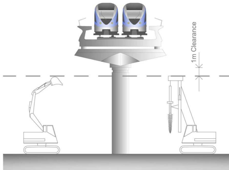
Figure 4.4: RA2.2 - Operation of equipment directly below Railway viaducts should keep minimum clearance from the structure
