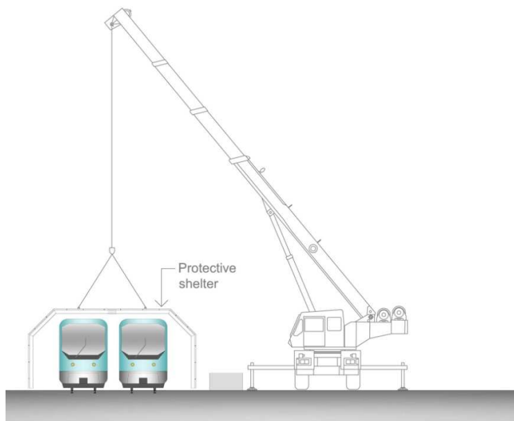
Figure 7.4: Site Preparation – Protection Shelter over Railway
