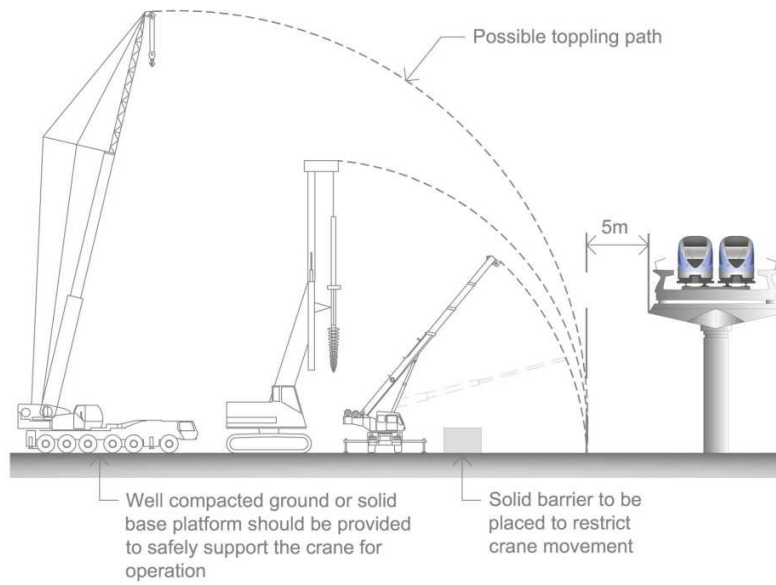
Figure 4.3: RA2.1 - Equipment should not operate within, or be able to collapse into, the area directly adjacent to the Railway structure
