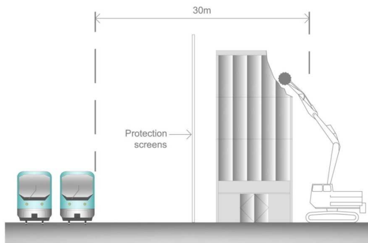
Figure 4.11: RA7 - Robust safety protection screens should be provided during demolition works within the Railway Protection Zone
